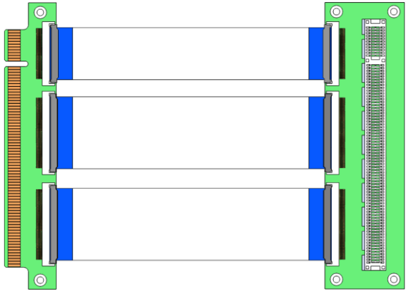
P27S-P27F (KZ-B23x16-DB23)
