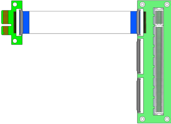
P21S-P27F (KZ-B23x1-DB23)
